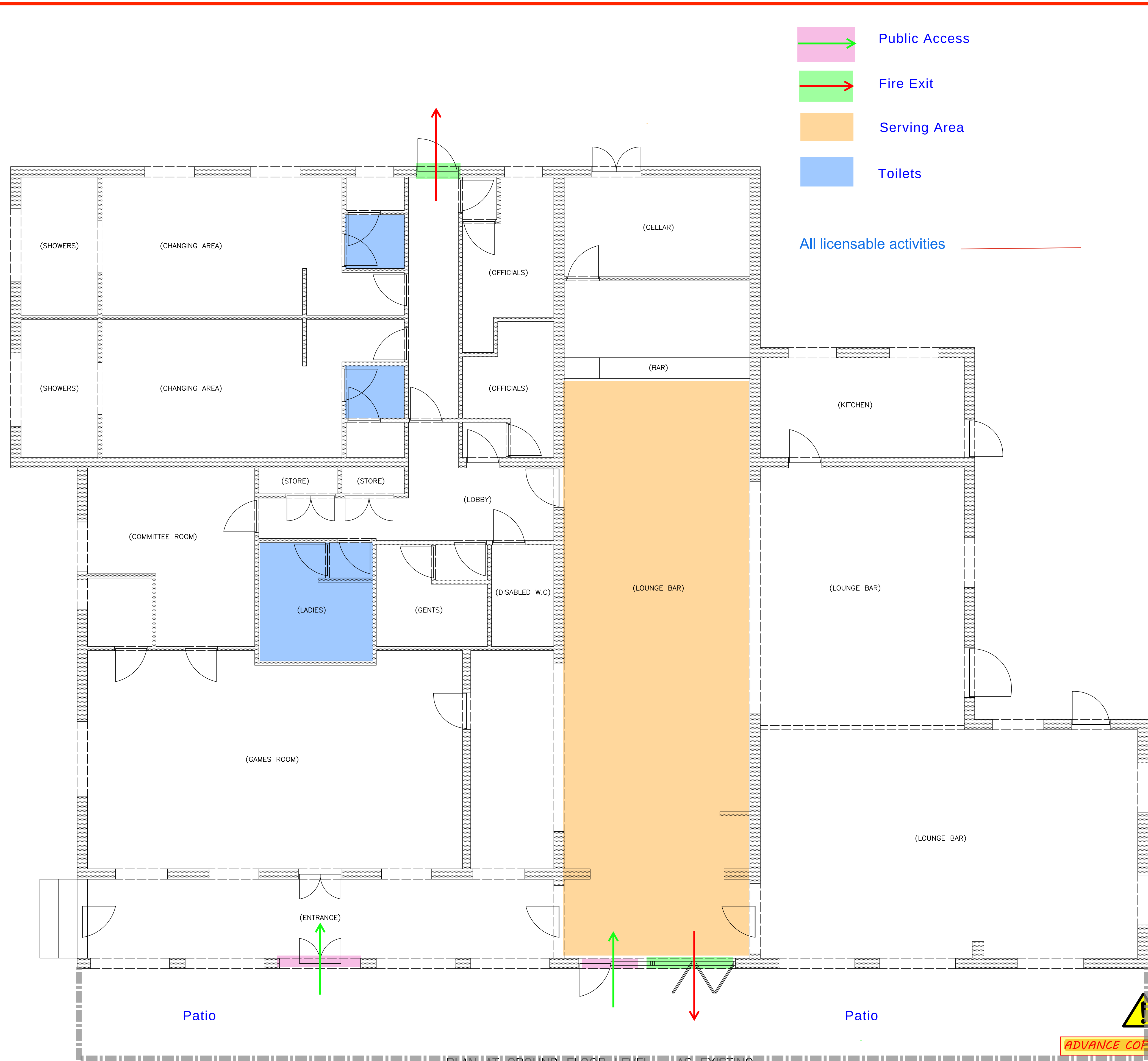
PLAN AT GROUND FLOOR LEVEL - AS EXISTING
