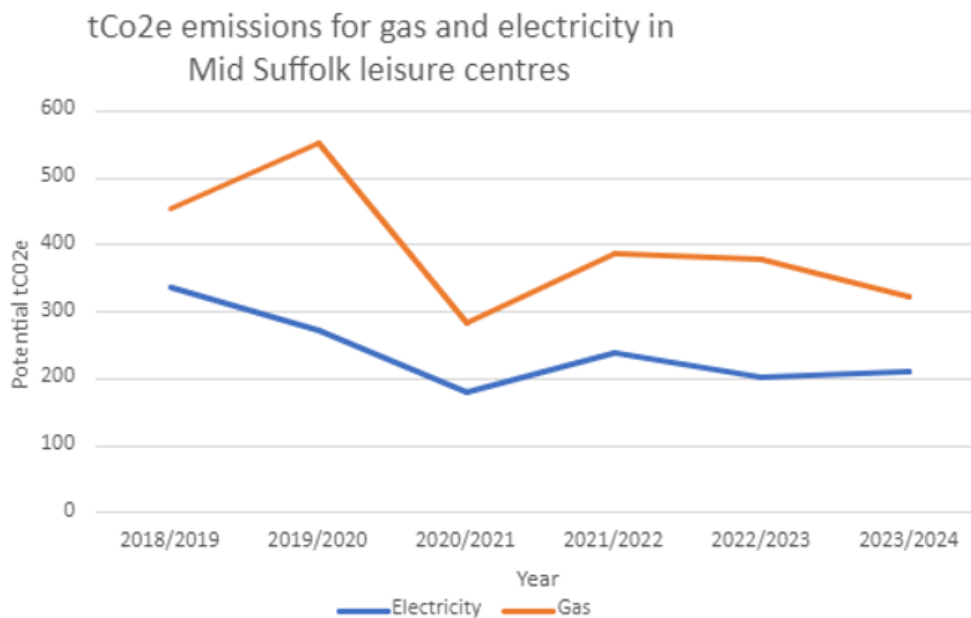
Graphic 7: Change in Co 2 e emissions for gas and electricity energy used at leisure centres in Mid Suffolk
