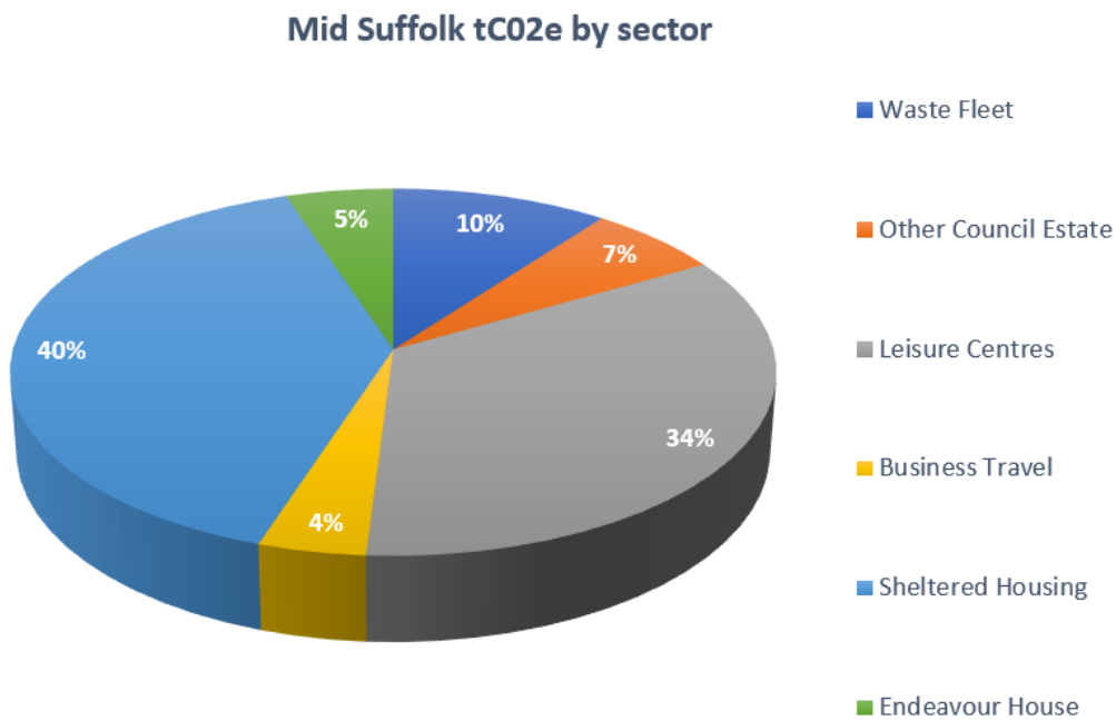
Graphic 5: Pie chart showing the % CO 2 e produced by each sector in Mid-Suffolk in 2023/24
