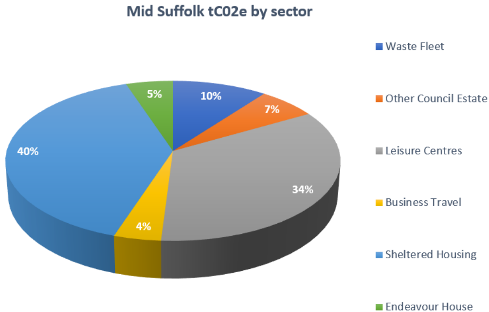
Graphic 2: Pie chart showing the % CO 2 e produced by each sector in Mid-Suffolk in 2023/24
