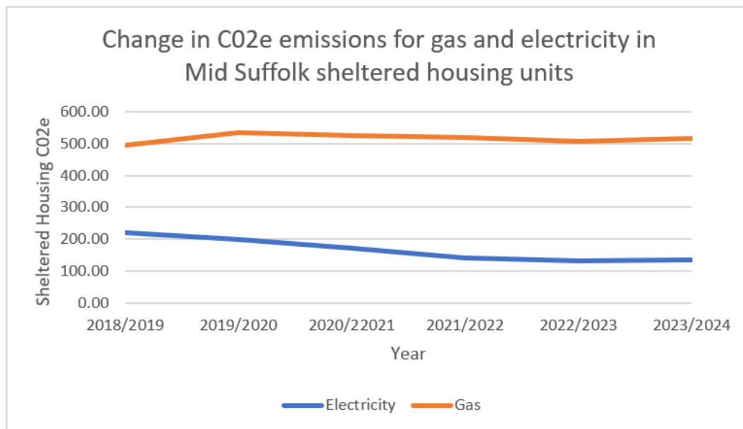
Graphic 6: Change in Co 2 e emissions for gas and electricity in Mid Suffolk sheltered housing units
