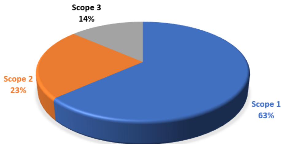
Graphic 4: Pie chart showing the % emissions in Mid Suffolk by Scope
