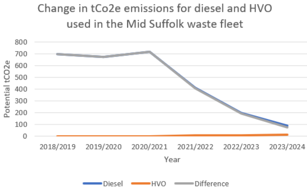
Graphic 8: Change in Co 2 e emissions for diesel and HVO used in the waste fleet
